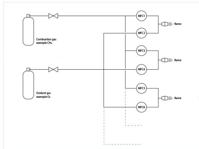
Schematical drawing
