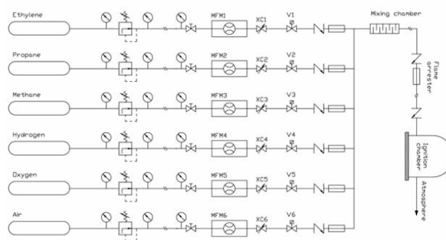
Flow scheme
