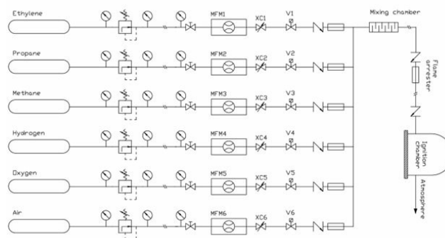
Flow scheme
